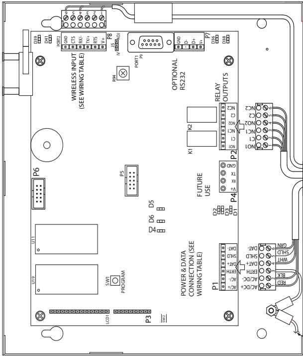
Drawing 16. Wireless multiplexer wiring
